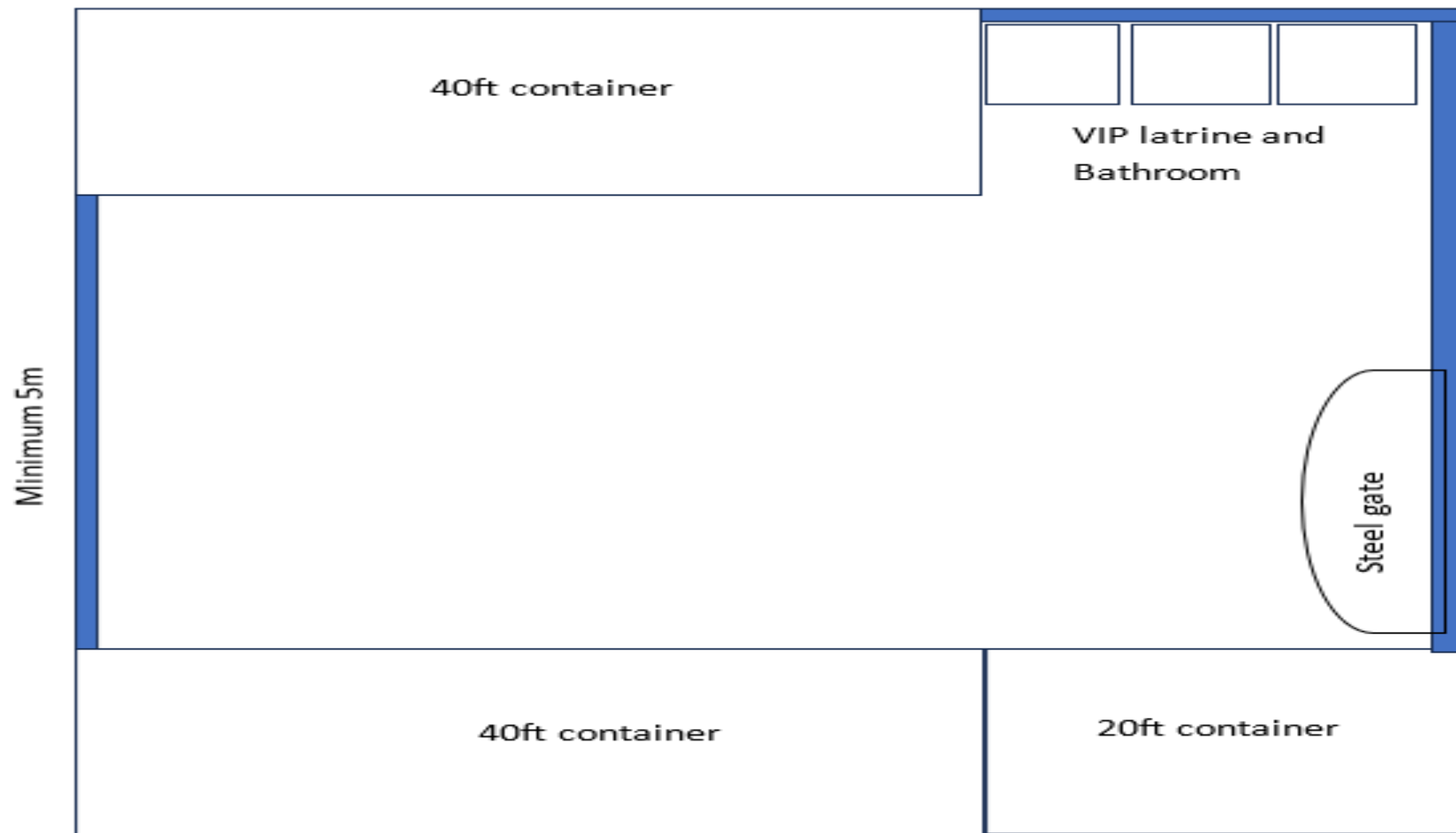
Figure 1: Site layout
